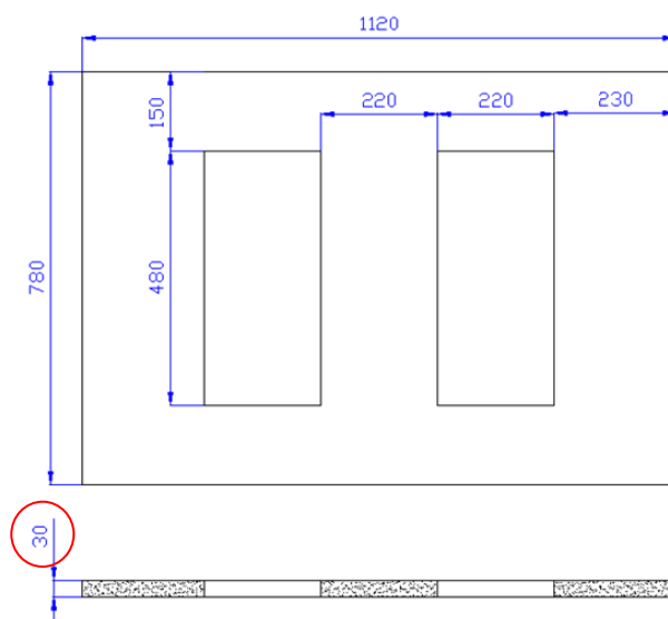
TAMPO (1.120mm x 780mm)
